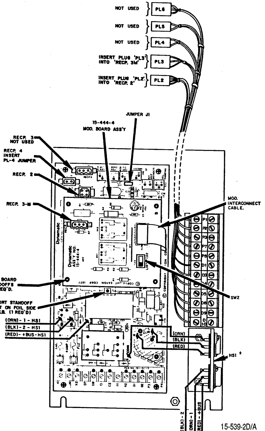
Model 4050 Controller Panel with Modification Board 15-444-4 Adjustable Brake
