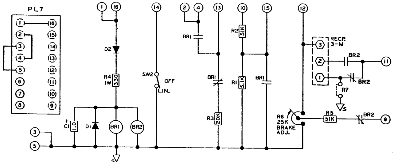
Adjustable Brake Modification PCB 15-444-4
